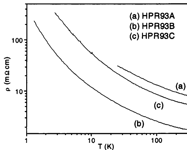
FIG. 7. Temperature dependent resistivity of all three fibers after 1150 °C anneal. High T metallic behavior is lost, and the slope d\rho/dT continues to increase as T \rightarrow 0 (divergent behavior).
