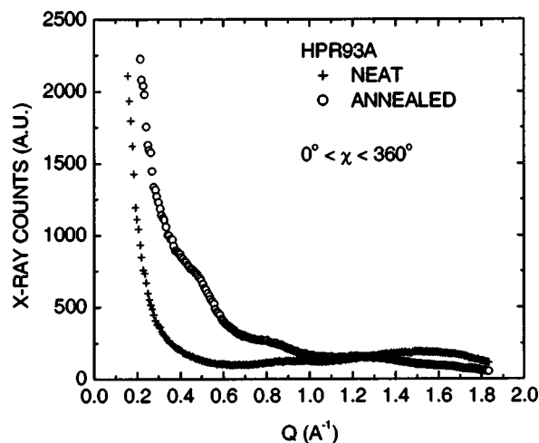
FIG. 1. Wide-angle x-ray scattering from neat and annealed fiber HPR93A. Samples are in transmission geometry. Powder profiles are obtained by azimuthal integration of the 2D data.
