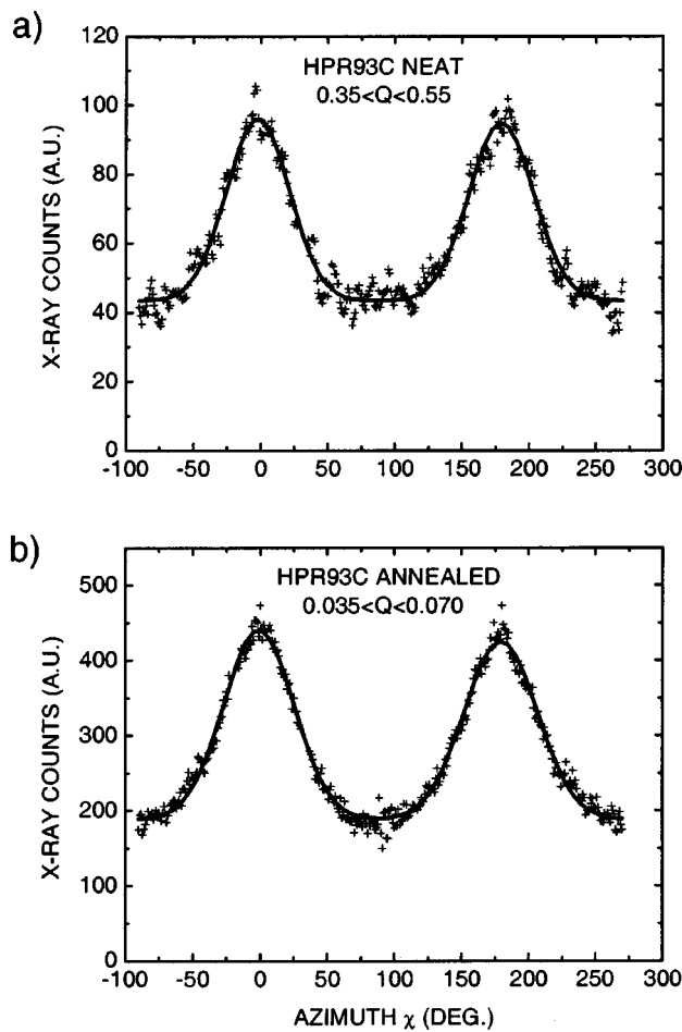
FIG. 2. Background-subtracted x-ray counts, summed over different Q intervals every 1^\circ in \chi . Data are the symbols; fits to two Gaussians plus a constant are the smooth curves. (a) Neat HPR93C, 0.35 < Q < 0.55 \text{ \AA}^{-1} centered at the (1,0) rope Bragg peak which is not visible in the data; (b) annealed HPR93C, 0.035 < Q < 0.070 \text{ \AA}^{-1} in the purely diffuse regime. Gaussian FWHMs are nearly equal, 55^\circ and 58^\circ , respectively, while the unoriented “background” is larger at low Q .
