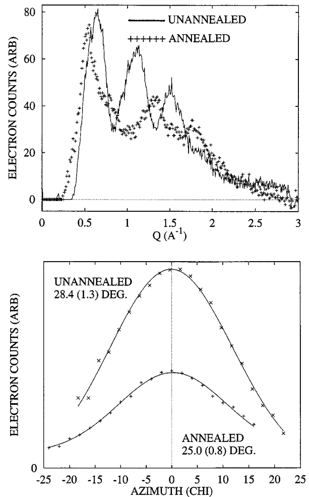
FIG. 2. Top: Equatorial intensity profiles ( Q \parallel H ) from electron diffraction recorded before and after in situ annealing of the thin H -aligned film at 800^\circ\text{C} . These are equivalent to powder profiles of the 2D triangular rope lattice since many ropes are sampled. The Q scale was calibrated using a polycrystalline gold standard. Bottom: mosaic distributions derived from radial slices \pm 21^\circ about the equator (symbols) along with Gaussian fits (solid curves). Radial intensities were summed over the first diffraction maximum at each \chi .
